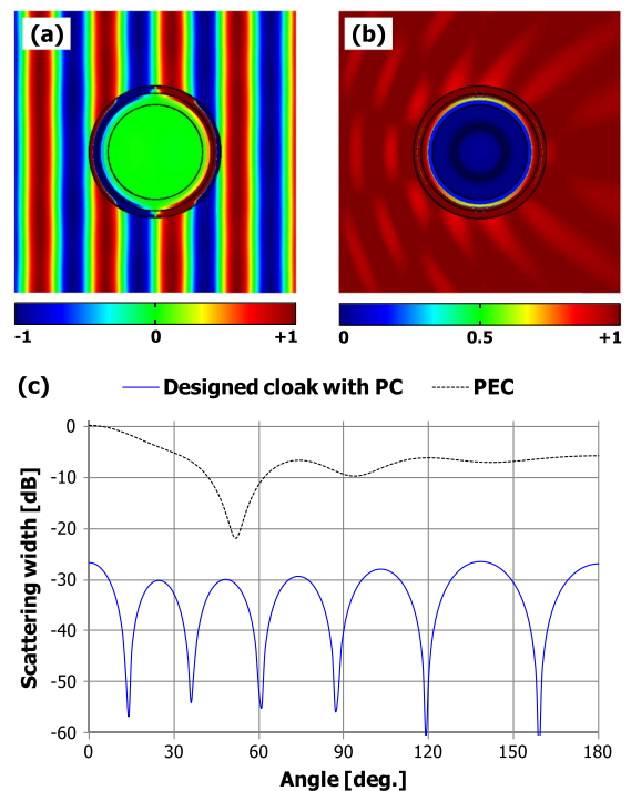
Fig. 3. (Color online) Calculated magnetic field distribution for the designed cloak with a PC (incident wavelength = 700 nm). (a) H_z field (Media 1). (b) H_z intensity. (c) Scattering widths for the designed cloak and an uncloaked PEC cylinder with R = 500 nm.
